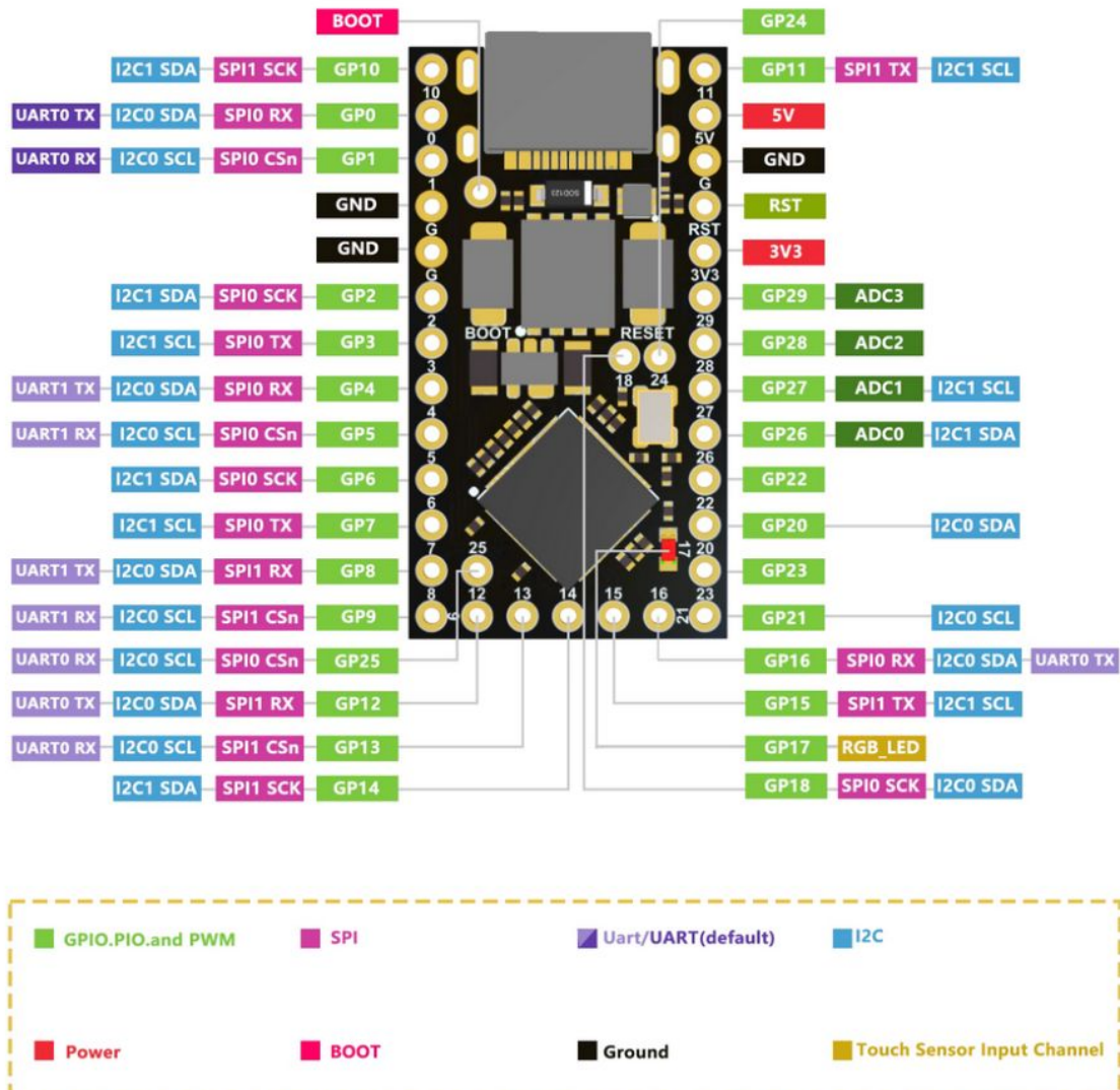
RP2040 ProMicro board
